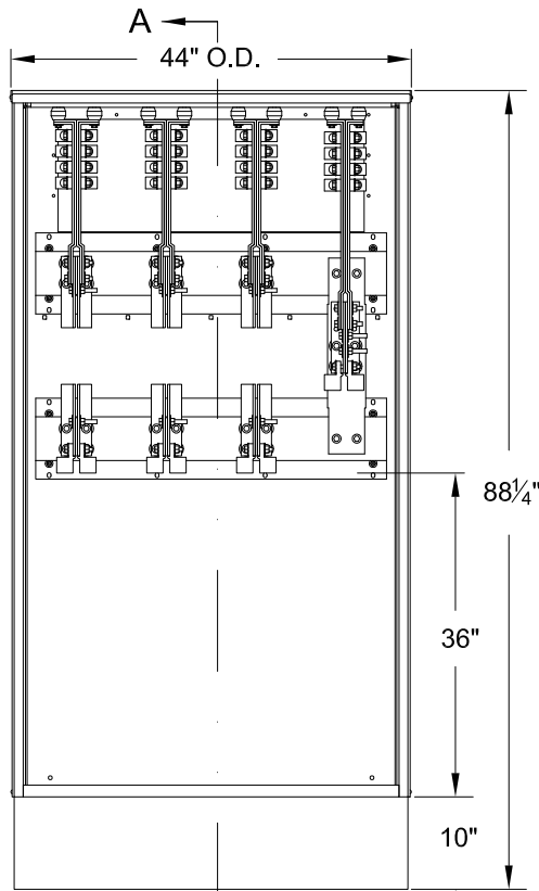
METERING TRANSFORMER COMPARTMENT (COVER REMOVED)
