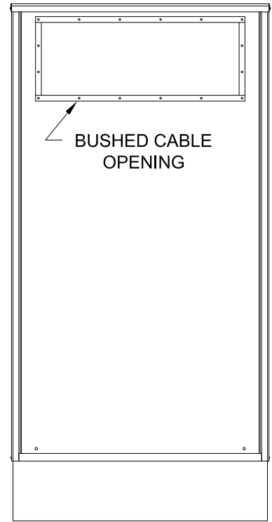
CONDUCTOR COMPARTMENT (COVER REMOVED)
