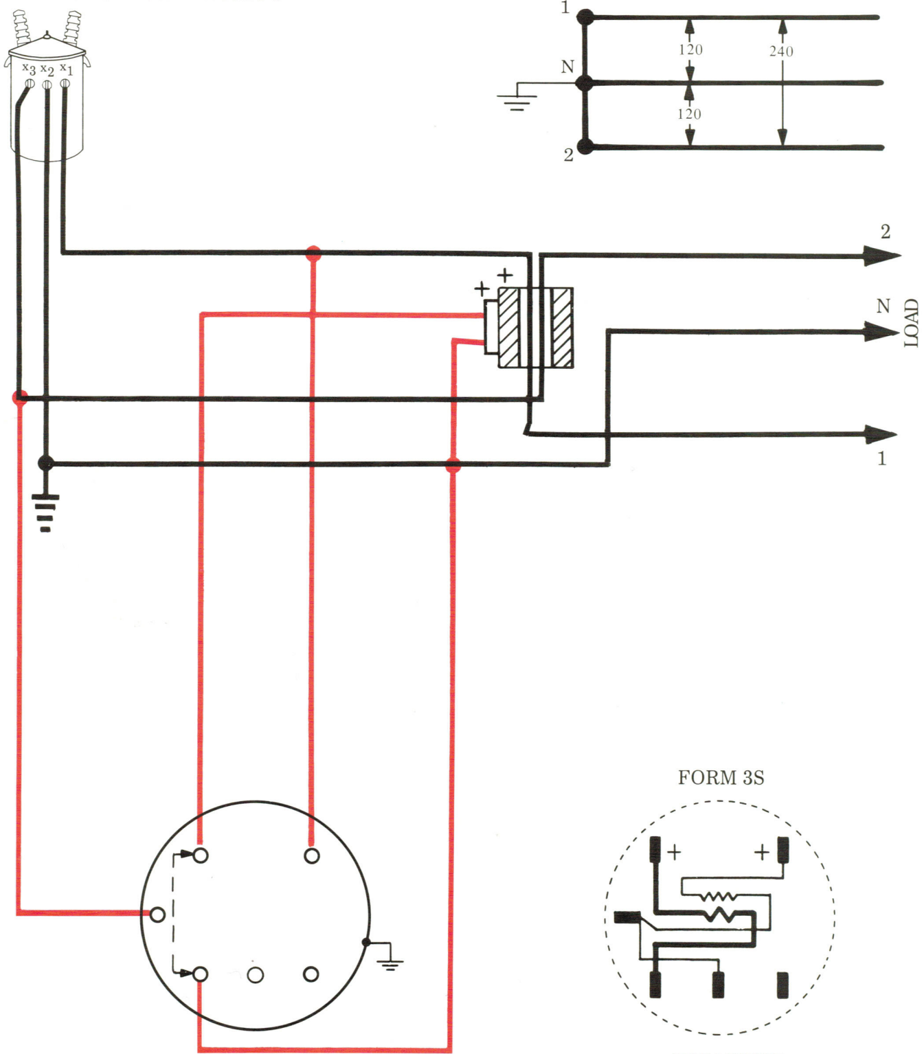
5-TERMINAL CIRCUIT CLOSING SOCKET FRONT VIEW
