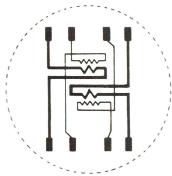
FORM 5S D5S-2 METER INTERNAL DIAGRAM FRONT VIEW
