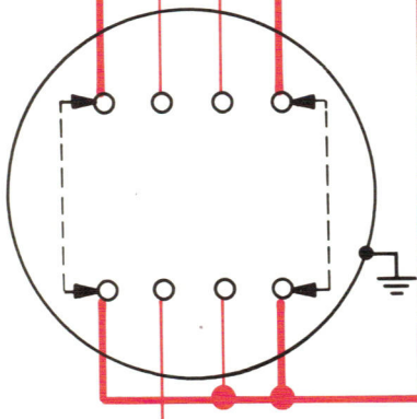
8-TERMINAL CIRCUIT CLOSING SOCKET, FRONT VIEW
