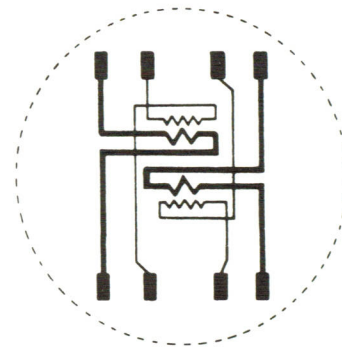
D5S-2 METER INTERNAL DIAGRAM FRONT VIEW
