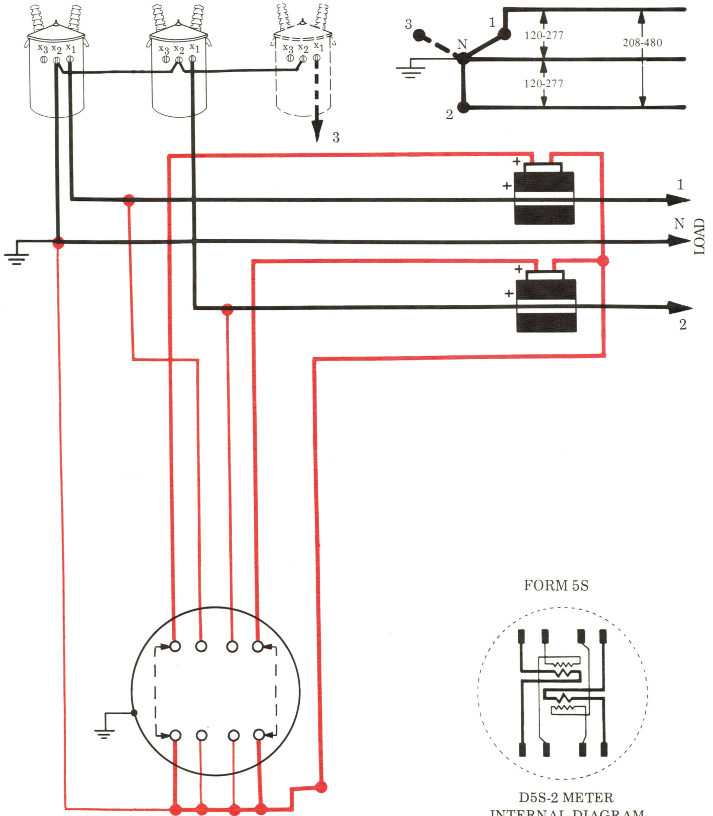
8-TERMINAL CIRCUIT CLOSING SOCKET
